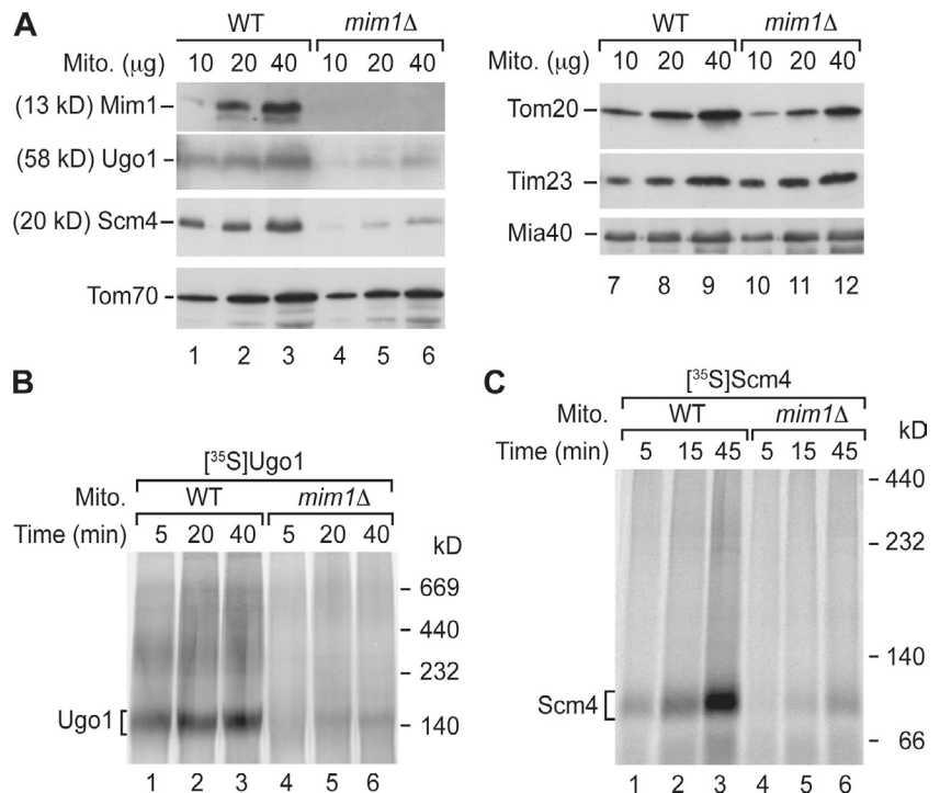
Figure 2. Assembly of multispanning outer membrane proteins is inhibited in the absence of Mim1. (A) Mitochondria (Mito.) were analyzed by SDS-PAGE and Western blotting. WT, wild type. (B and C) ^{35}\text{S} -Ugo1 or Scm4 was imported into wild-type and mim1 \Delta mitochondria. Mitochondria were lysed with digitonin and analyzed by blue native electrophoresis.
